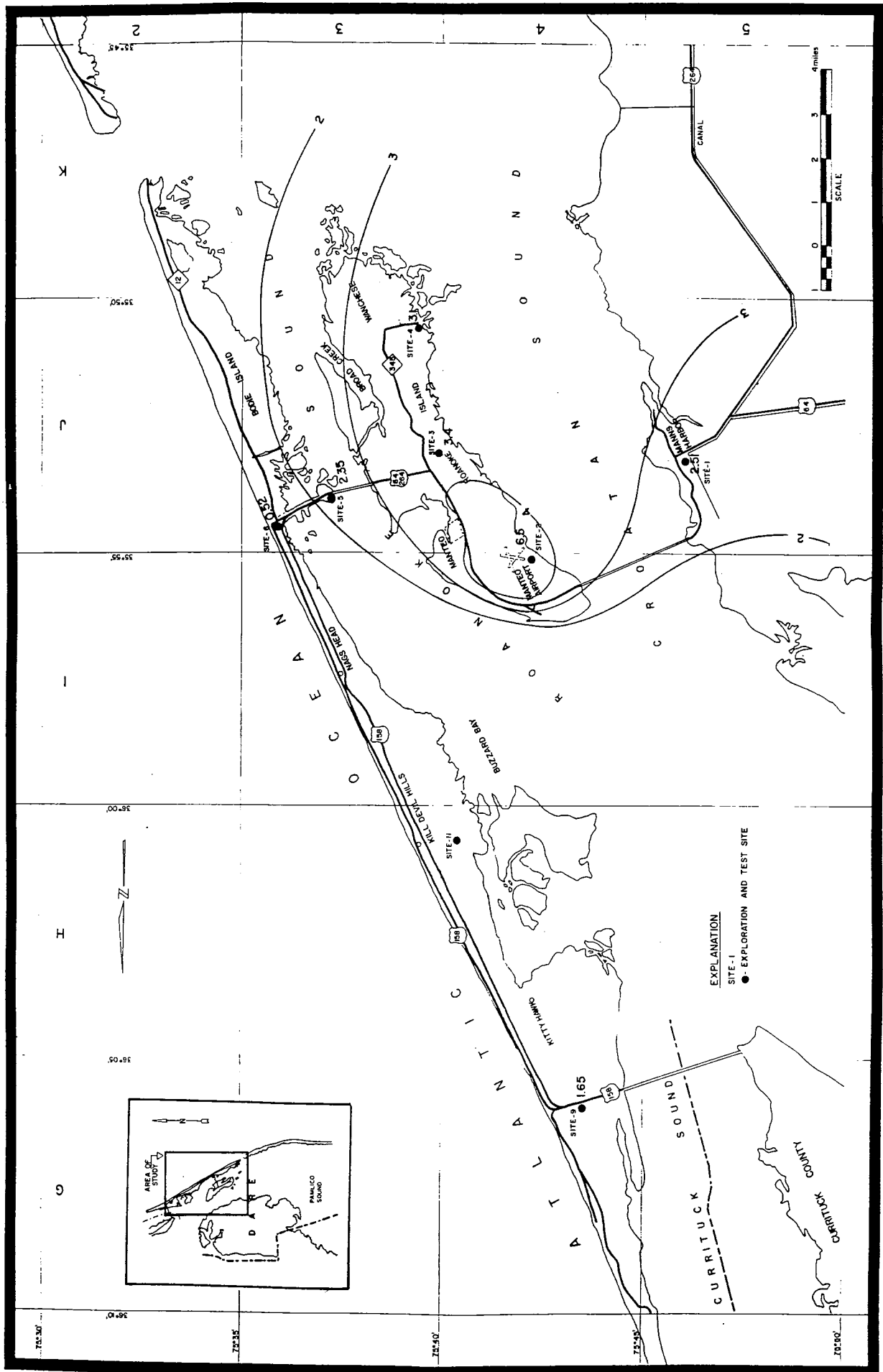
FIGURE 10. - PIEZOMETRIC SURFACE OF PRINCIPAL AQUIFER - JANUARY 1973
