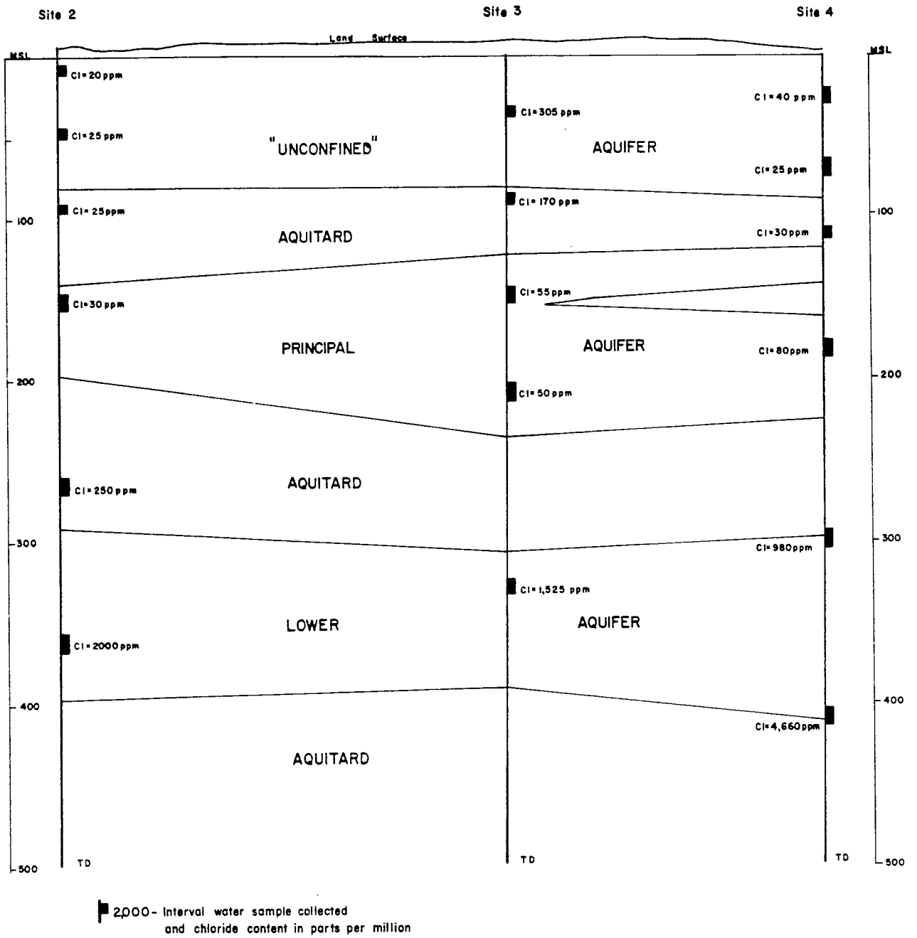
FIGURE 3.- HYDROGEOLOGIC CROSS-SECTION, SITE 2 TO SITE 4
