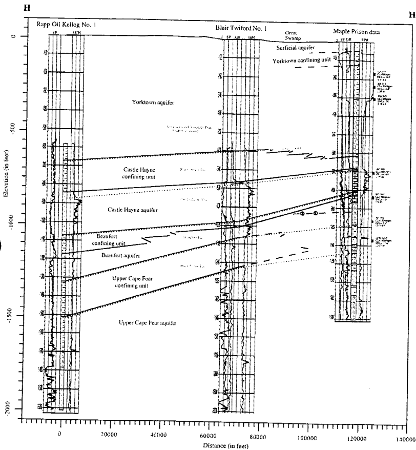
PLATE A-10 South to North Hydrogeologic Cross-Section H-H' through Currituck County, NC
