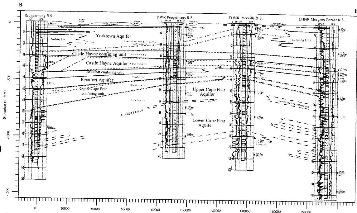
PLATE A-3 South to North Hydrogeologic Cross-Section B-B' through Chowan, Perquimans, Pasquotank Counties, NC
