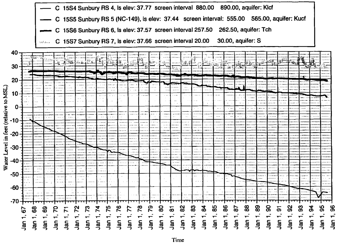
FIGURE 4 Hydrograph of NCDENR Sunbury Research Station
