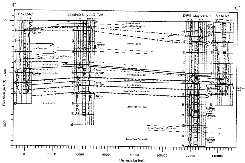
PLATE A-4 South to North Hydrogeologic Cross-Section C-C' through Pasquotank, Camden, and Currituck Counties, NC and Chesapeake City, VA
